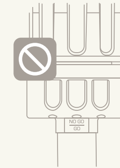
INCORRECT installation shown via NO-GO gauge
